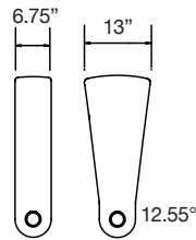
Straight & Wedge Arm Connectors
