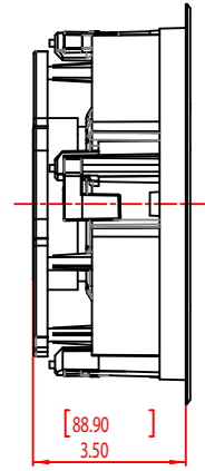
MOUNTING DEPTH
