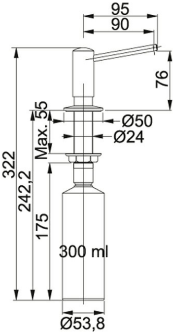
Technical Drawing
