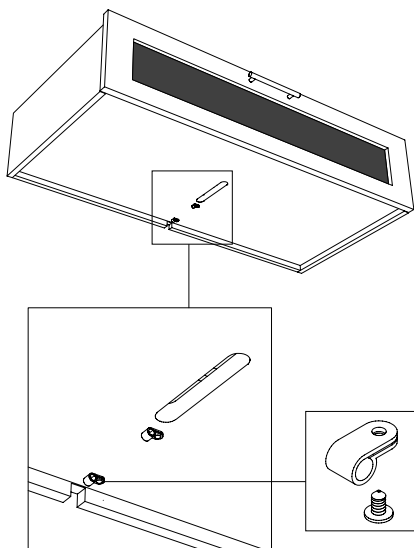
Wire Clip/Screw
