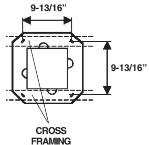
TOP VIEW OF SUPPORT FRAME
