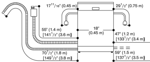
Connection dimensions for an 18" (45 cm) wide dishwasher
