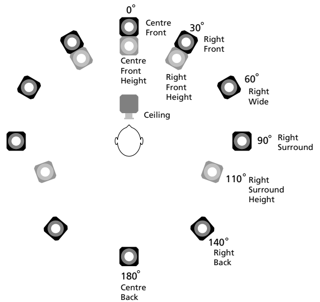
Figure 4.4: Loudspeaker positions associated with the speaker roles available in the television. The True Image processor delivers a unique output to each of these output channels.
