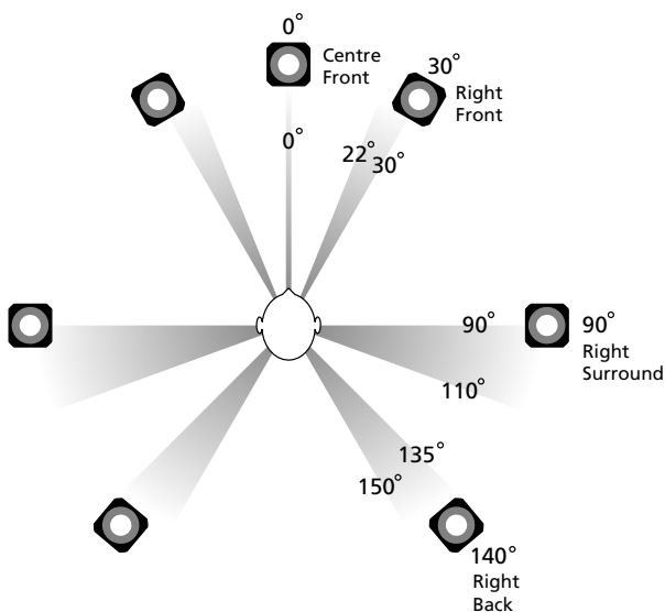
Figure 4.3: Recommended loudspeaker configuration for most 7.1 channel audio signals. The actual positions of the loudspeakers shows the reference placement used at Bang & Olufsen for testing and tuning.
