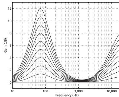
Figure 3.5: An example of the effect of the Loudness on the frequency response of the system at different volume settings. The lowest curve is for a high volume setting. The highest curve represents the response at a low volume setting. In this example, the Bass Max Boost is set to 12 dB and the Treble Max Boost is set to 9 dB.
