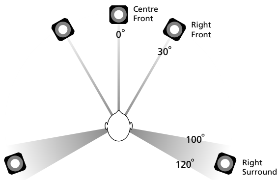
Figure 4.2: Standard loudspeaker configuration for 5.1 multi-channel audio. The actual positions of the surround loudspeakers at 110° shows the reference placement used at Bang & Olufsen for testing and tuning. Note that the placement of the subwoofer is better determined by your listening room's acoustics, but it is advisable to begin with a location near the centre front loudspeaker.
