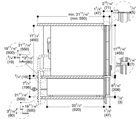
Side view WS 463 under BS, BM, CM
