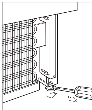
Front adjustment.
