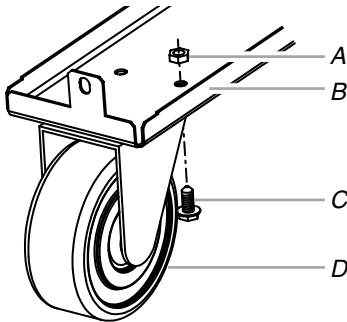
A. Self-locking nut B. Caster bracket C. \frac{5}{16} -18 x \frac{7}{8} " hex-head bolt D. Caster
