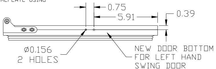
STRIKER PLATE HOLE LOCATION.
