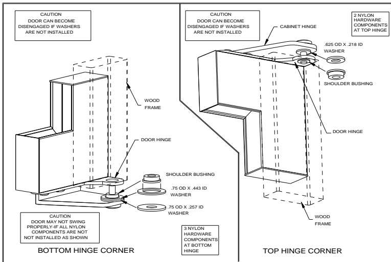
HINGE HARDWARE INSTALLATION DETAILS.
