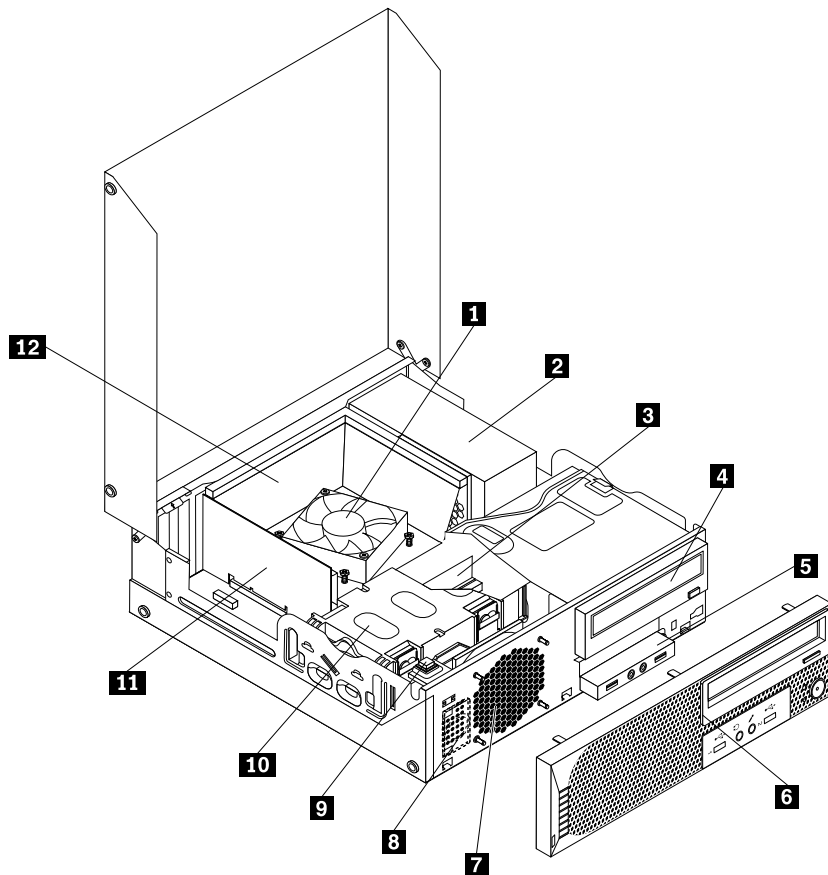
Figure 3. Component locations
