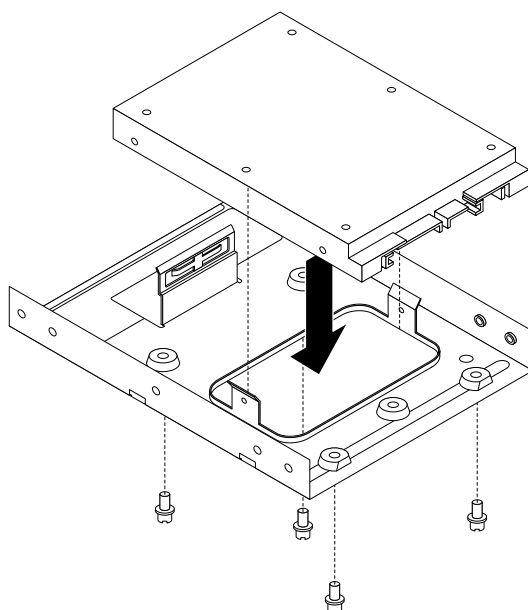
Figure 25. Installing the solid state drive into the adapter
