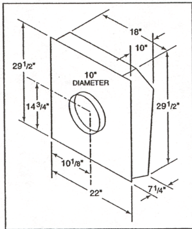
Remote blower dimensions – 1200 CFM (801642)
