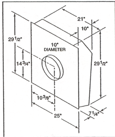
Remote blower dimensions – 1500 CFM (804701)
