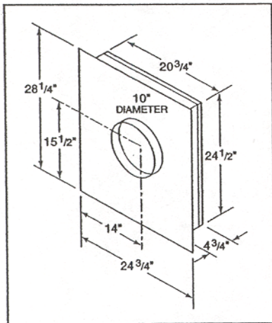
Remote blower dimensions – 600 CFM (801640) and 900 CFM (801641)
