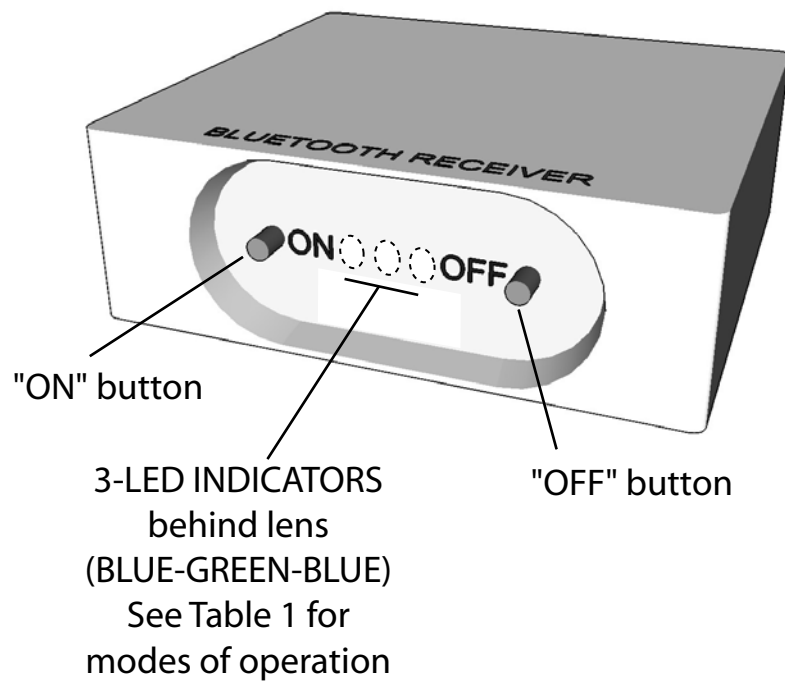
FRONT PANEL
