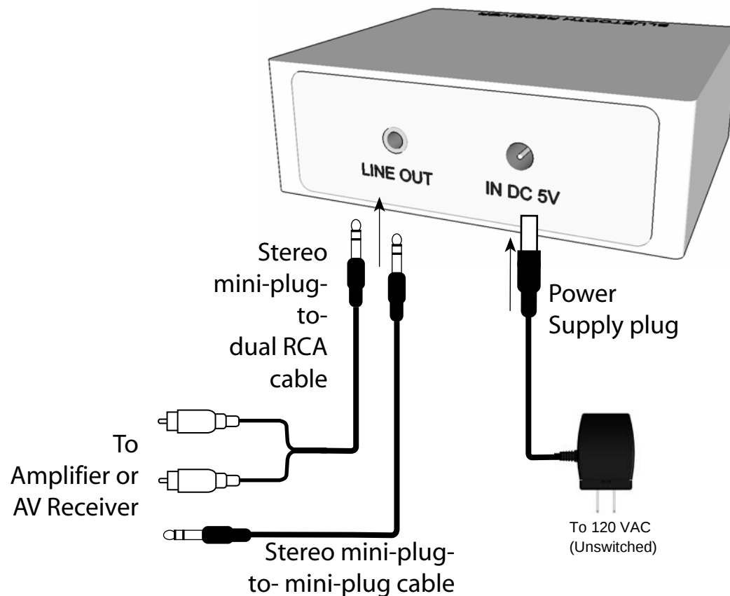
REAR PANEL
