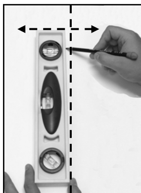
Masonry - Step 1
