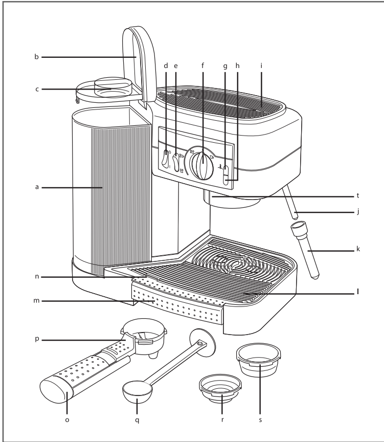
Fig 1, Capresso Café User Components
