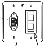
INLET FACEPLATE
