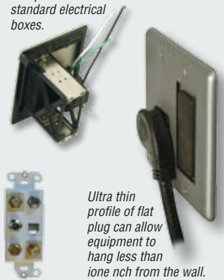
Decora Adapters can accommodate 6-port insert (insert not included)
