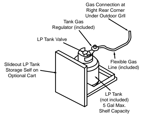
Installing the LP Tank in Cart
