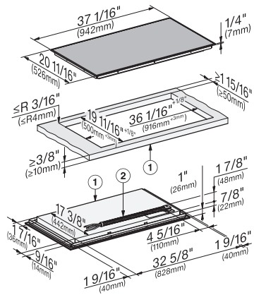
KM7747FR Diamond – frameless overlaying installation
