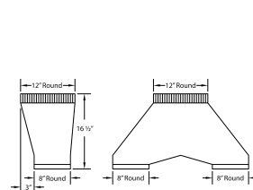
VP563 Transition (Optional) For B400 (Double B200 Dual Blowers)
