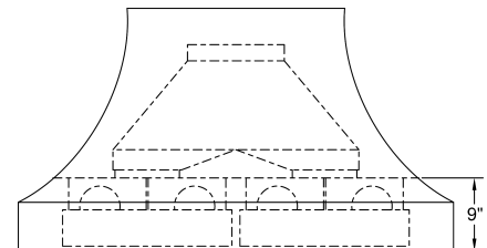
VP563 Standard Transition Installed (Front View)
