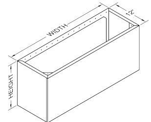
Wall Mount Duct Cover Models: WDCRND-*
