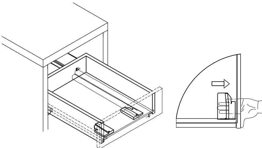
Unlatching the drawer
