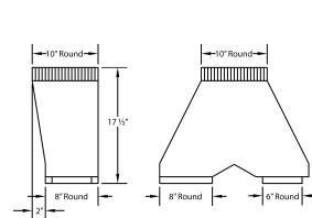
VP562 Transition (Optional) For B300 (B200 Dual Blower & B100 Single Blower)
