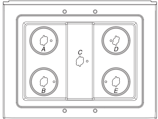
A. Standard burner - Propane gas orifice spud number 088 B. Power burner - Propane gas orifice spud number 117 C. Center burner - Propane gas orifice spud number 096 D. Simmer burner - Propane gas orifice spud number 068 E. Power burner - Propane gas orifice spud number 117
