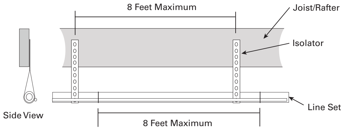
Isolation From Joist/Rafter
