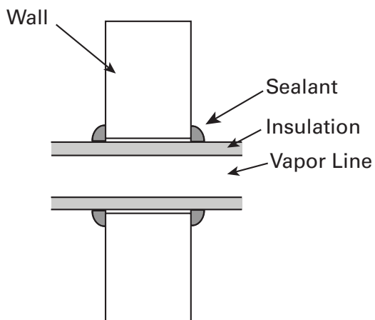
Isolation Through Wall
