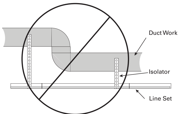
Isolation In Wall Spaces
