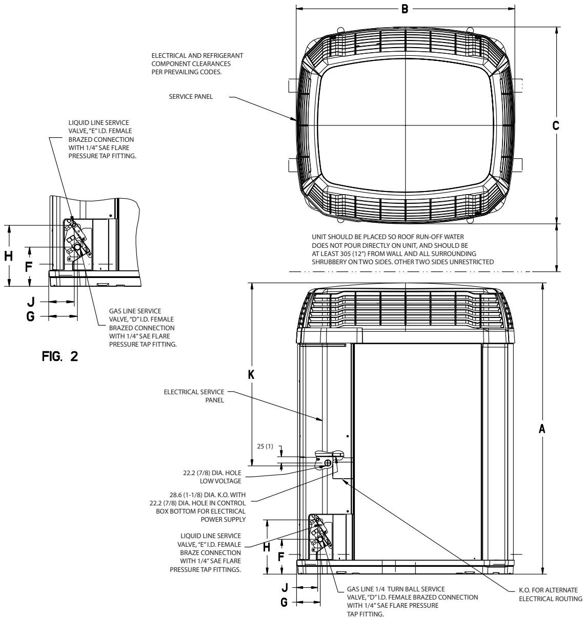
Figure 2. Dimensional drawing
