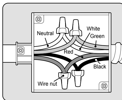
Junction Box
