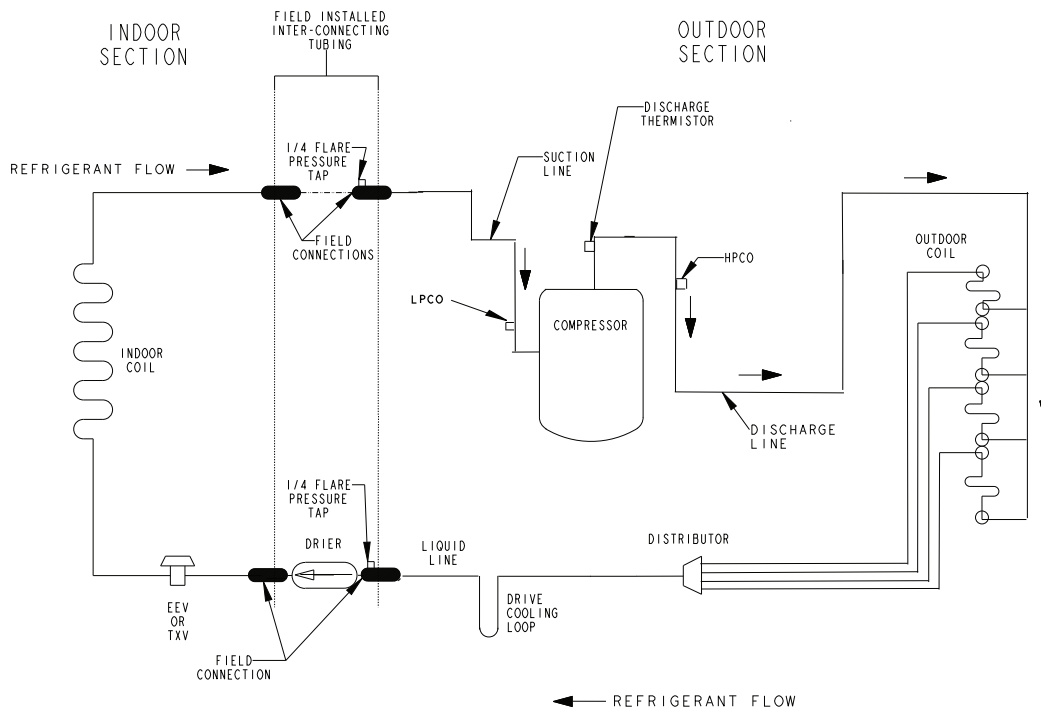
Figure 14. 2 ton and 3 ton A/C
