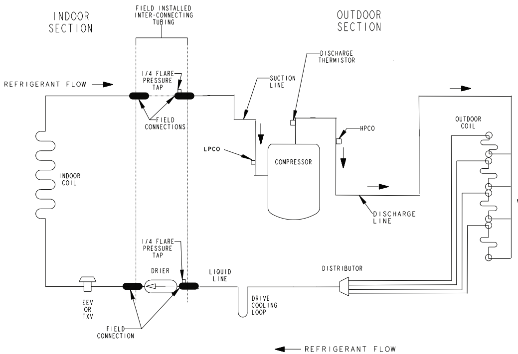
Figure 14. 2 ton and 3 ton A/C
