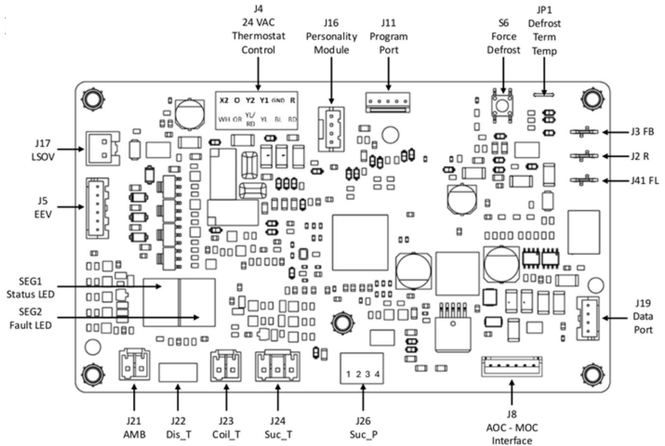
Figure 9. LED indicators
