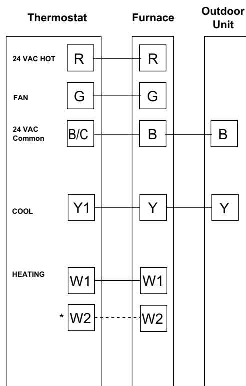
Figure 24. With furnace
