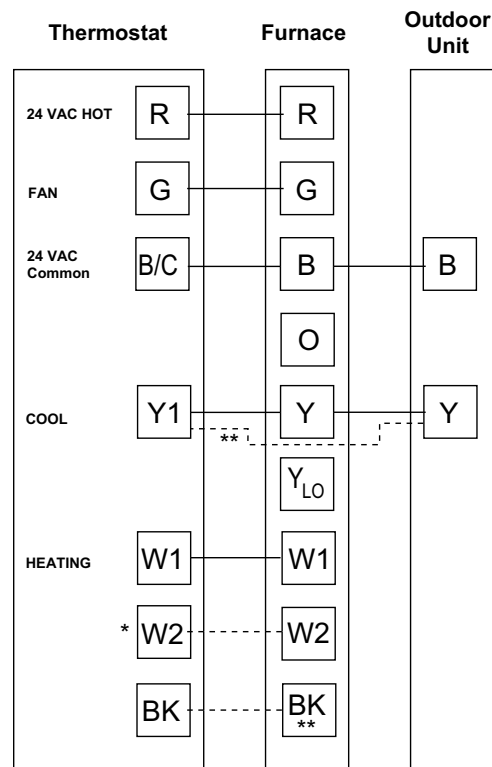
Figure 25. With variable speed furnace
