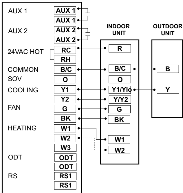
Figure 26. 2-stage AC thermostat
