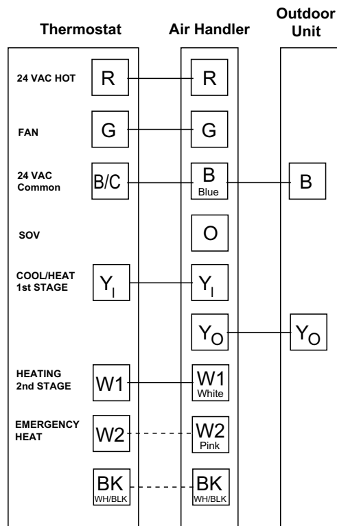
Figure 24. With furnace
