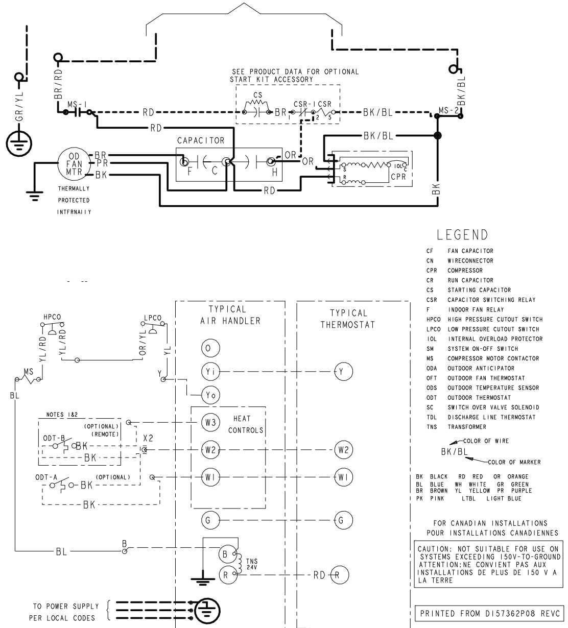
Figure 1. Models 5TTX6018A, 024A, 030A, 036A, 042A, and 048A
