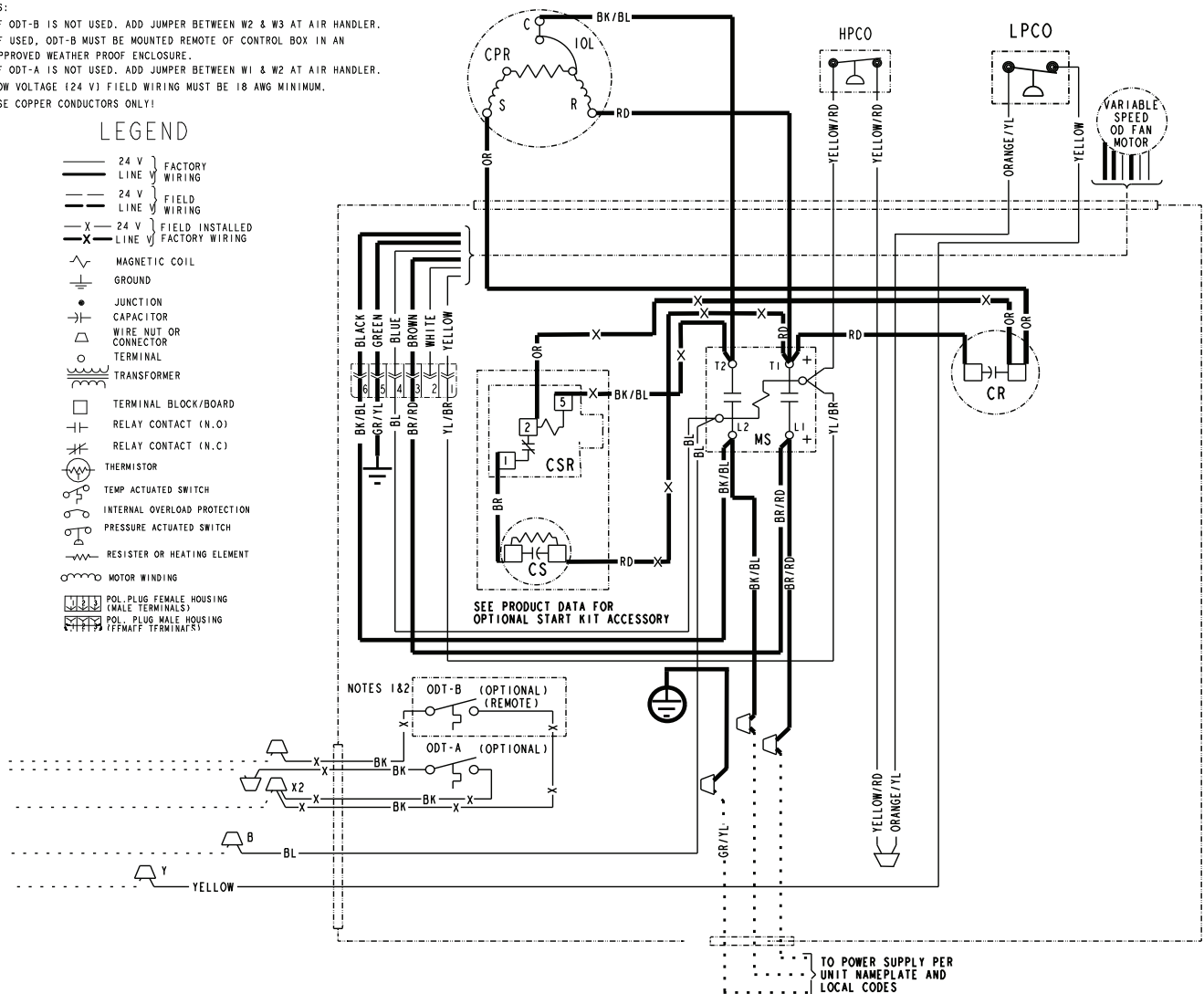
Figure 4. Model 5TTX6060A
