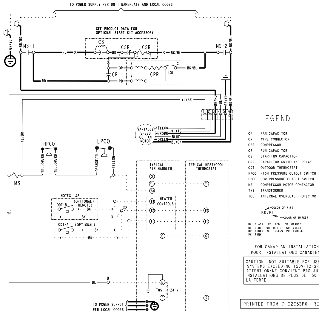
Figure 3. Model 5TTX6060A
