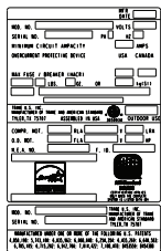
Figure 33. Nameplate location
