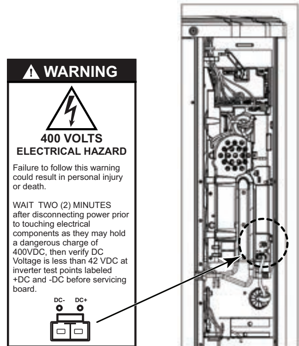
Figure 1. Warning label
