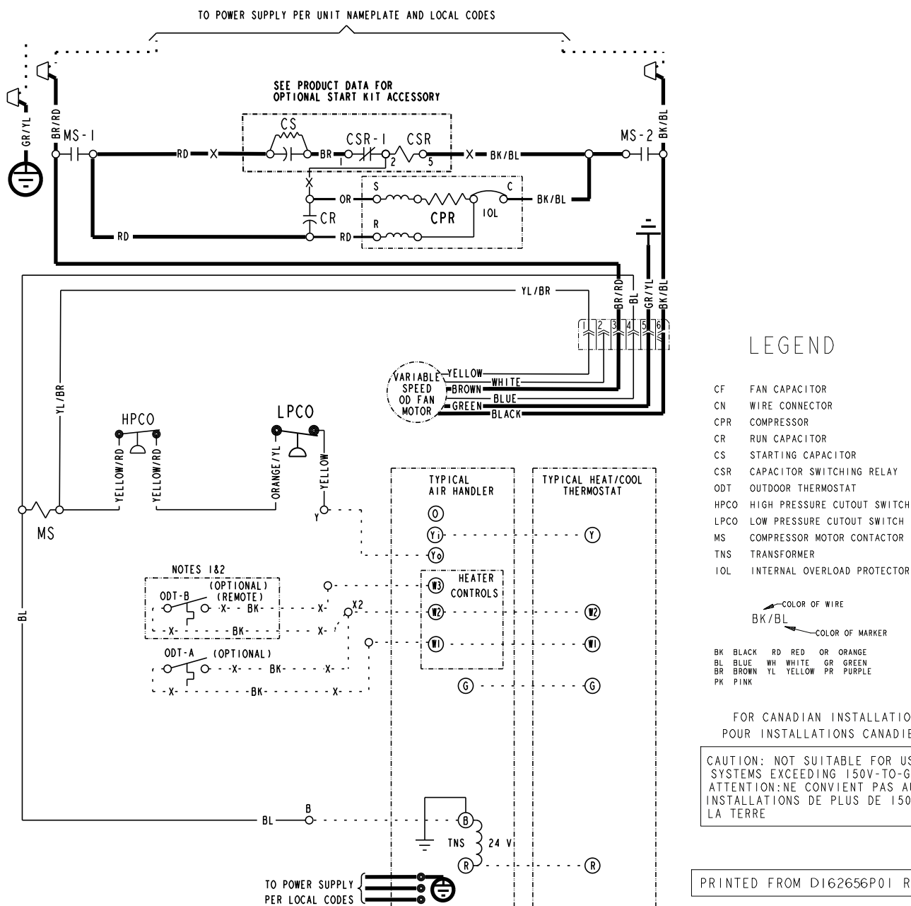
Figure 3. 060A Models
