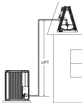
Figure 28. Refrigerant line total length and lift
