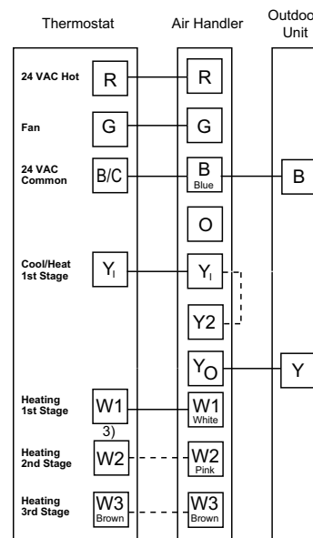
Figure 24. Single stage, AC, 5TEM5
