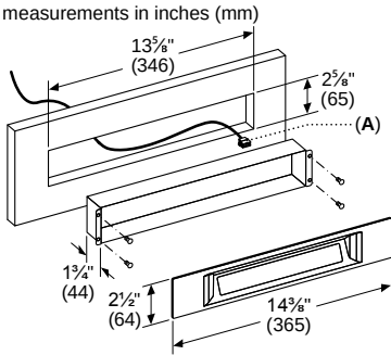
A: DBus Cable length: 30 feet (9180 mm)
