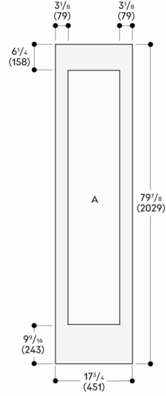
Niche width 18" (457 mm)
