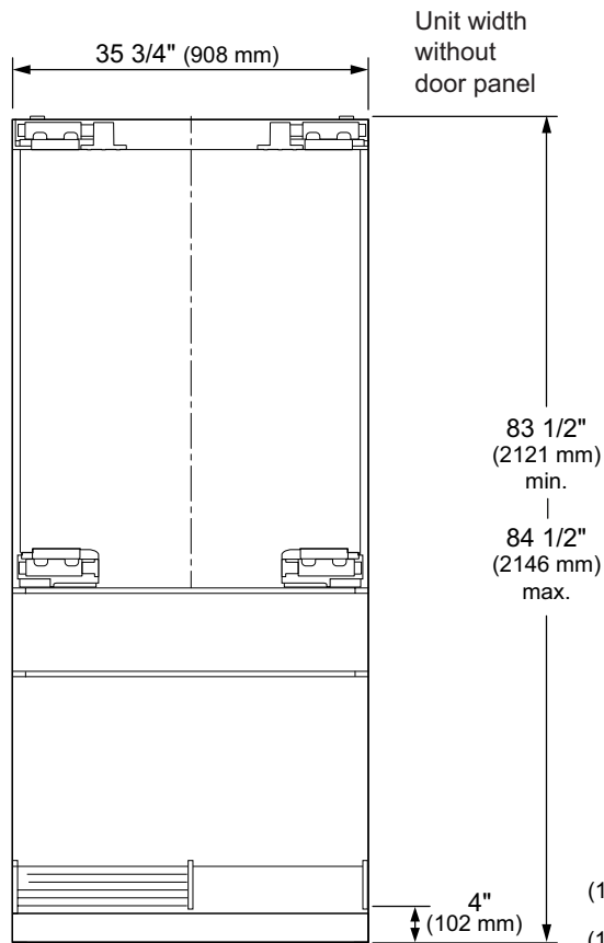
FRONT VIEW
