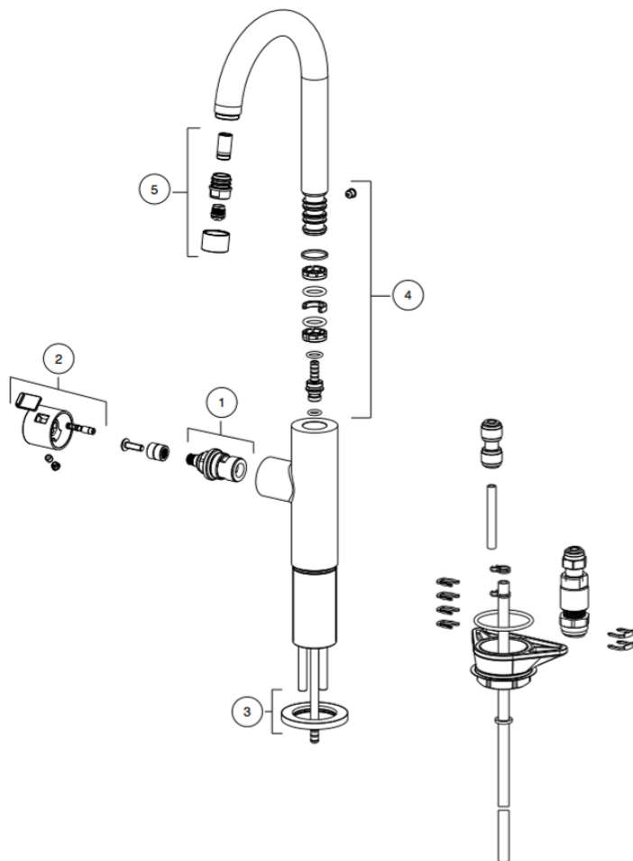
Tap Maris Lario Filtration MB
