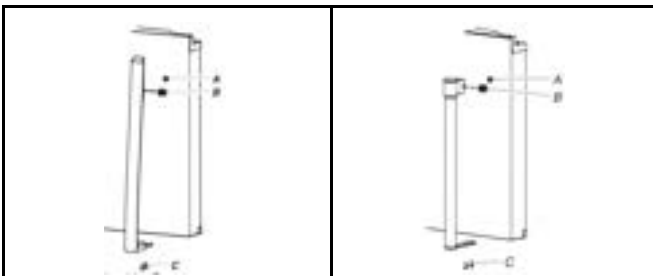
A. Shoulder screw B. Setscrew C. Flat-head handle screws
