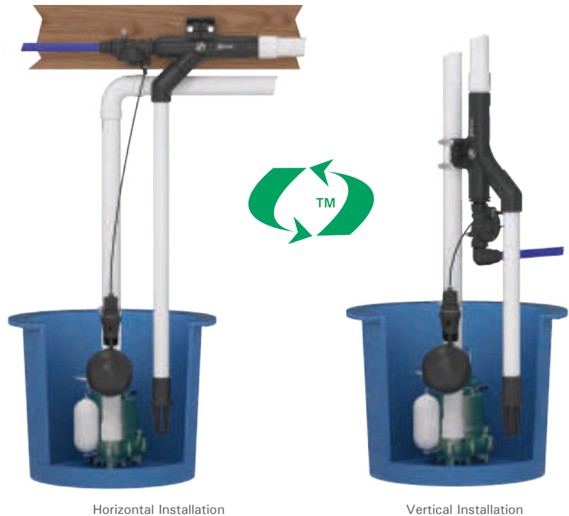
Horizontal Installation
