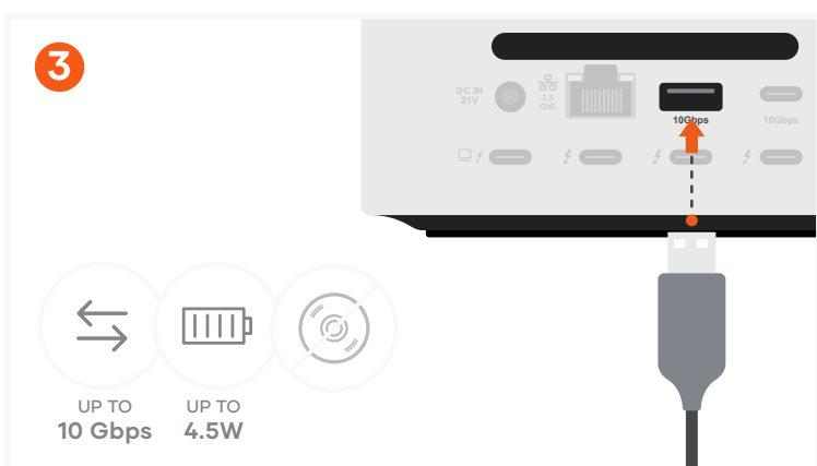
USB-A Port supports data transfer (10Gbps) and charging (4.5W).
