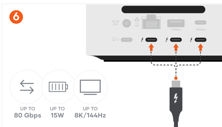
3x Thunderbolt 5 Ports.
