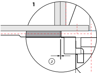
ADJACENT CABINET
