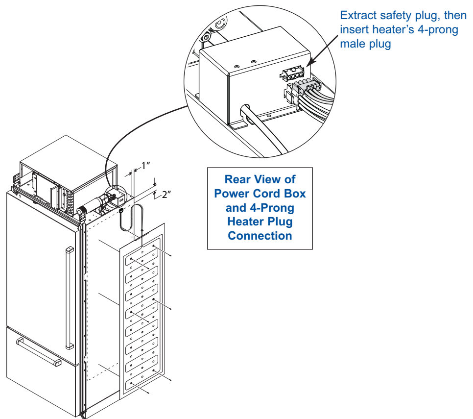
Figure 1. Heater Installation
