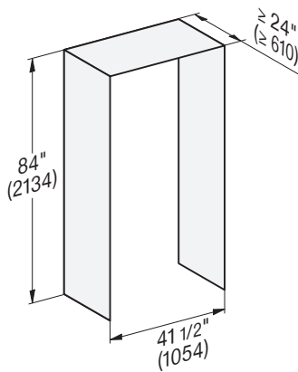
framed cabinet
