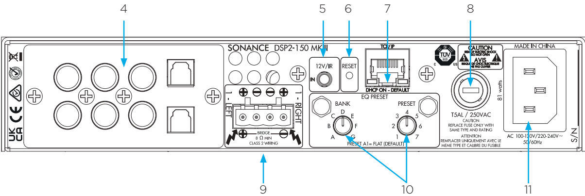
Figure 2: DSP 2-150 MKIII Two-Channel Power Amplifier Rear Panel
