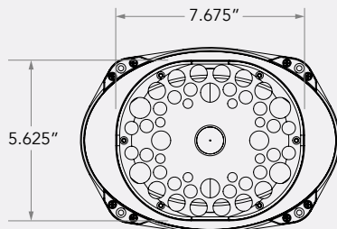
WAVEGUIDE DIMENSION FOR HOLE CUT
