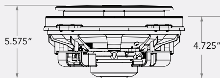
WAVEGUIDE DIMENSION FOR HOLE CUT
