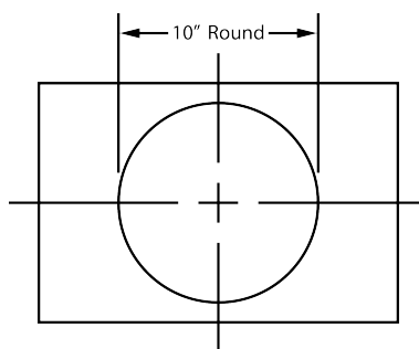
900 CFM B200 Dual &amp; B100 Single Blower (Top View)
