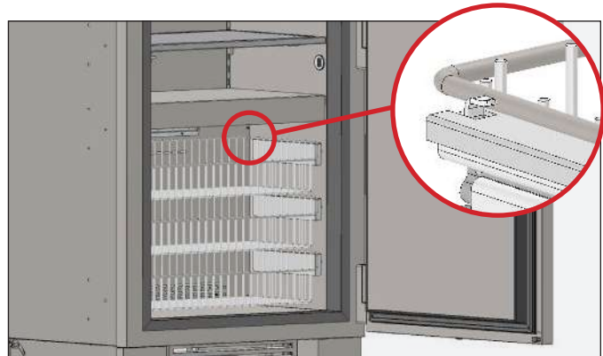
FIG. 3. Be sure the drawer sits under the rear tabs
