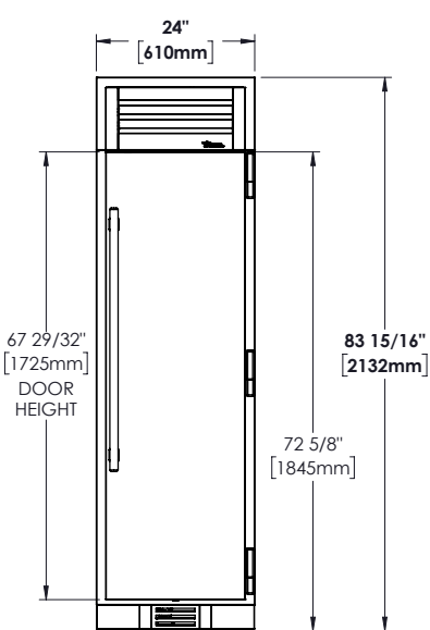
TR-24 – FRONT VIEW
