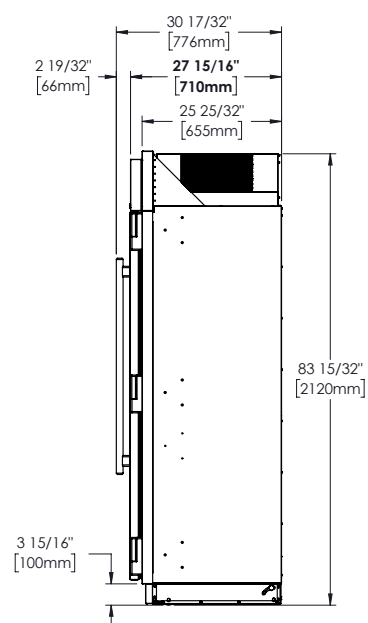
TR-24 – SIDE VIEW
