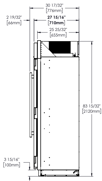
TR-30 – SIDE VIEW
