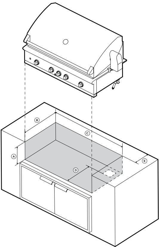
ISO VIEW
